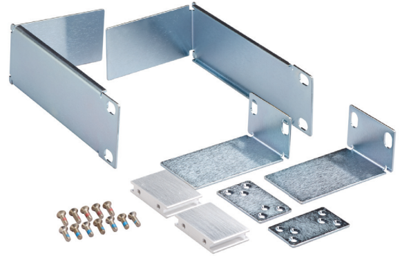
Figure 6. Remote Spectrum Monitor MS27101A-001 Rack-Mount Bracket Kit
